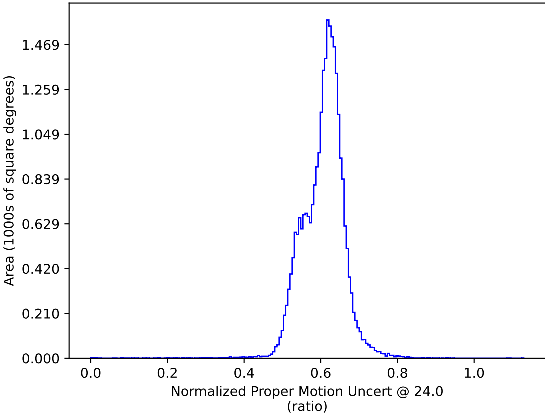
too_elab_r64_d2_griz_v3.4_10yrs : Normalized Proper Motion Uncert @ 24.0
