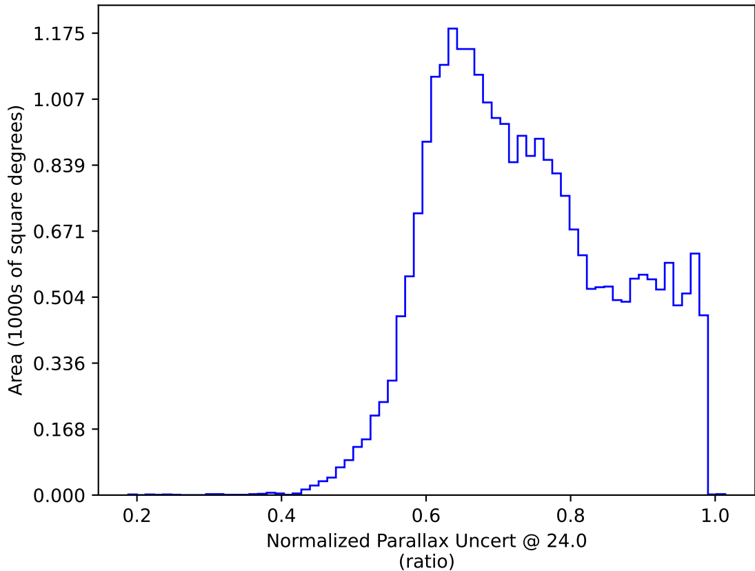
too_elab_r64_d2_griz_v3.4_10yrs : Normalized Parallax Uncert @ 24.0
