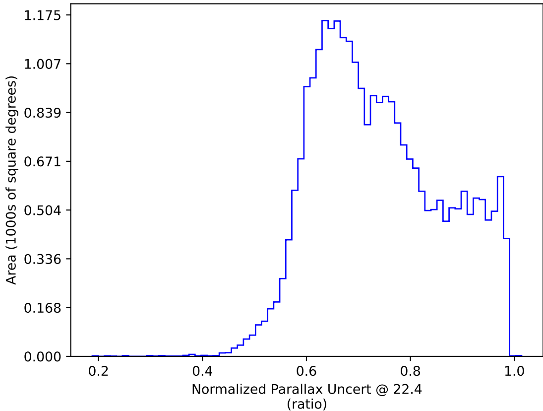
too_elab_r64_d2_griz_v3.4_10yrs : Normalized Parallax Uncert @ 22.4
