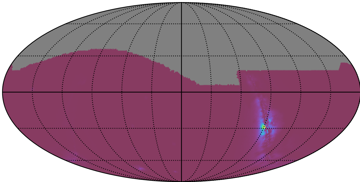
too_elab_r64_d2_griz_v3.4_10yrs : NlcPoints
