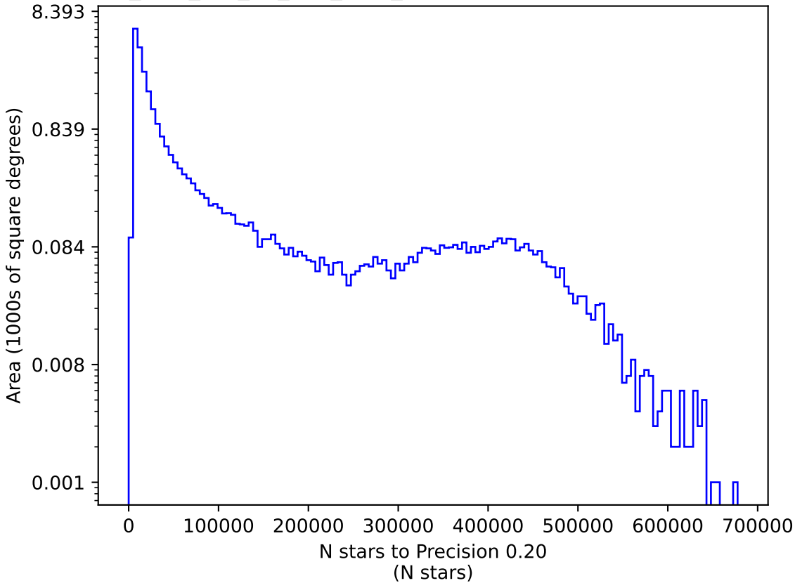
too_elab_r64_d2_griz_v3.4_10yrs z: N stars to Precision 0.20
