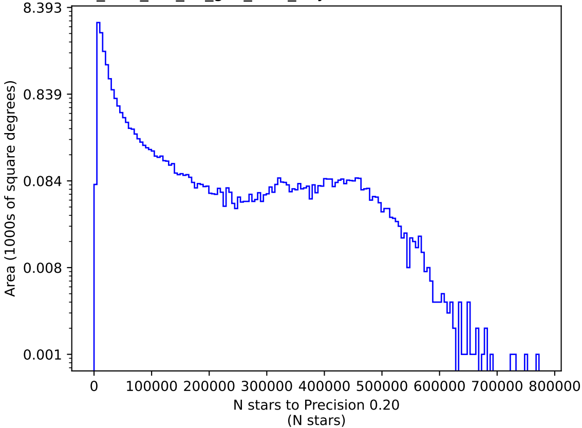
too_elab_r64_d2_griz_v3.4_10yrs i: N stars to Precision 0.20
