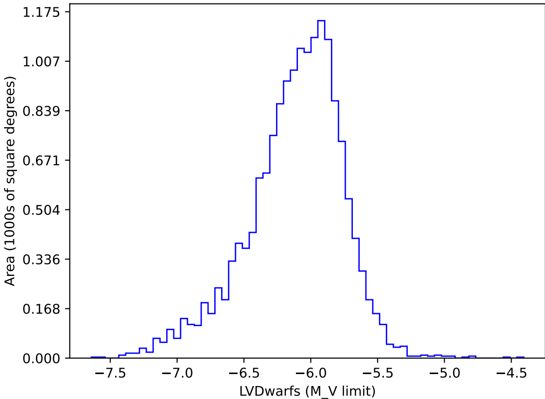
too_elab_r64_d2_griz_v3.4_10yrs gi: LVDwarfs
