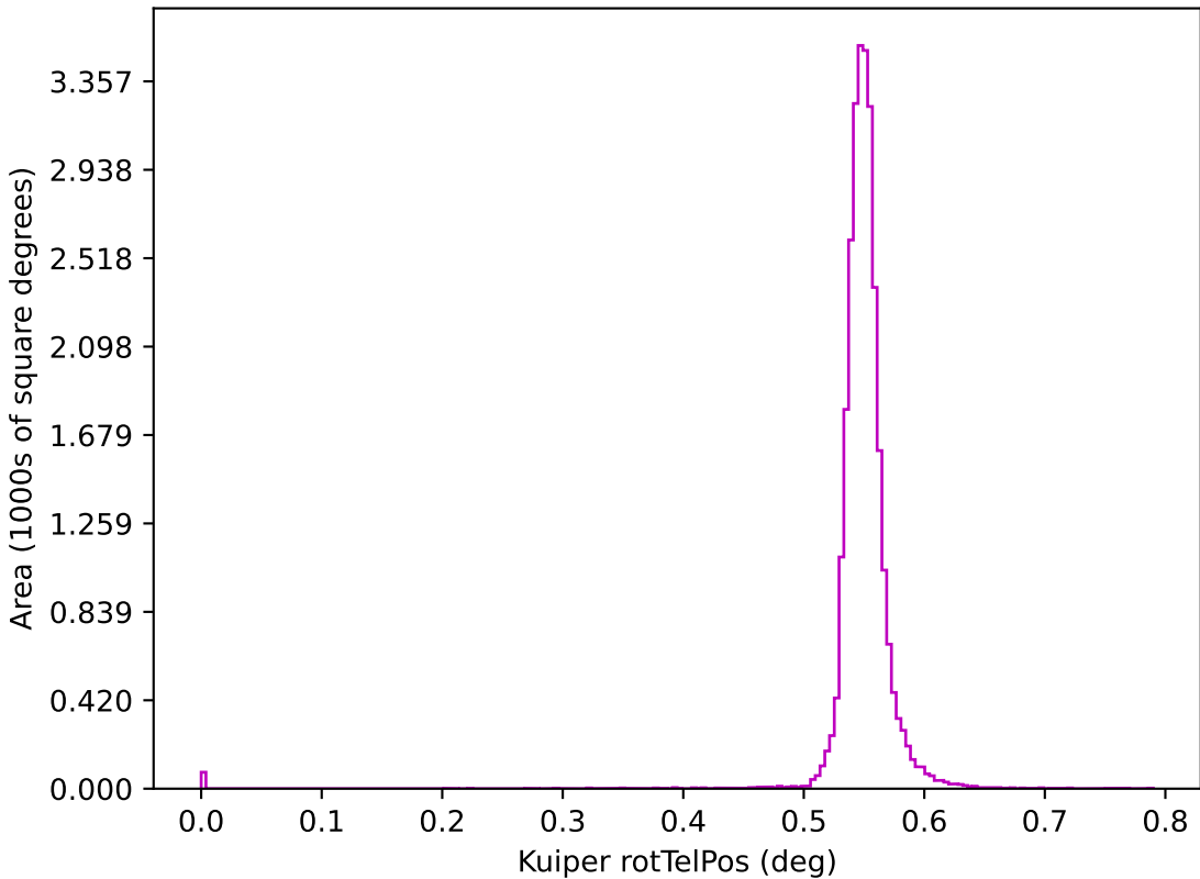
too_elab_r64_d2_griz_v3.4_10yrs z: Kuiper rotTelPos
