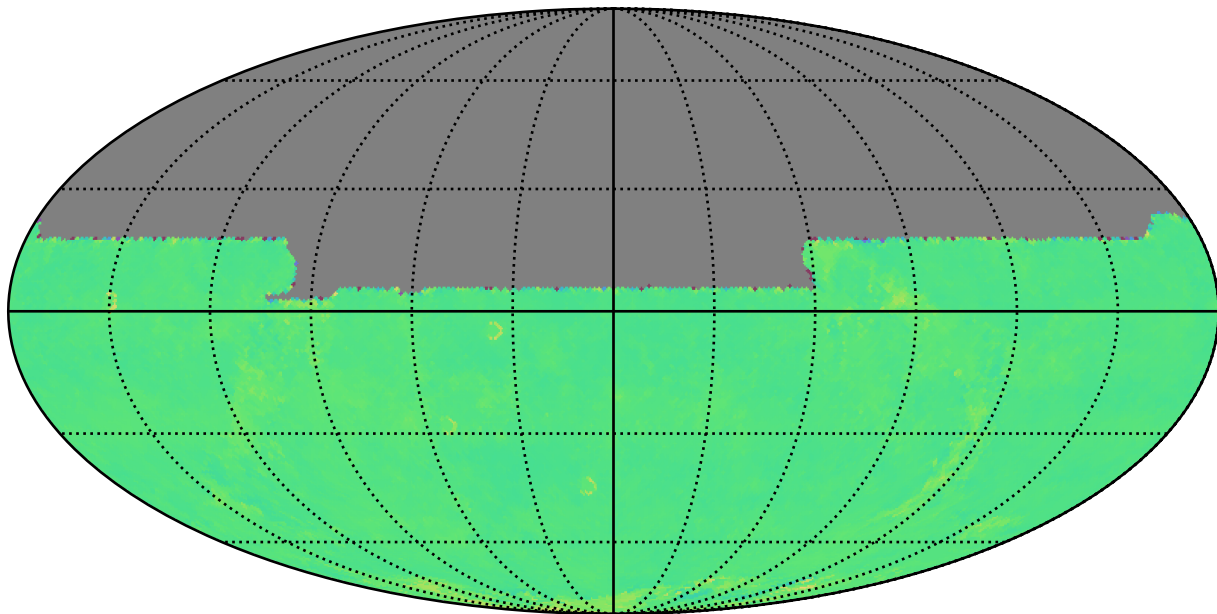
too_elab_r64_d2_griz_v3.4_10yrs y: Kuiper rotTelPos
