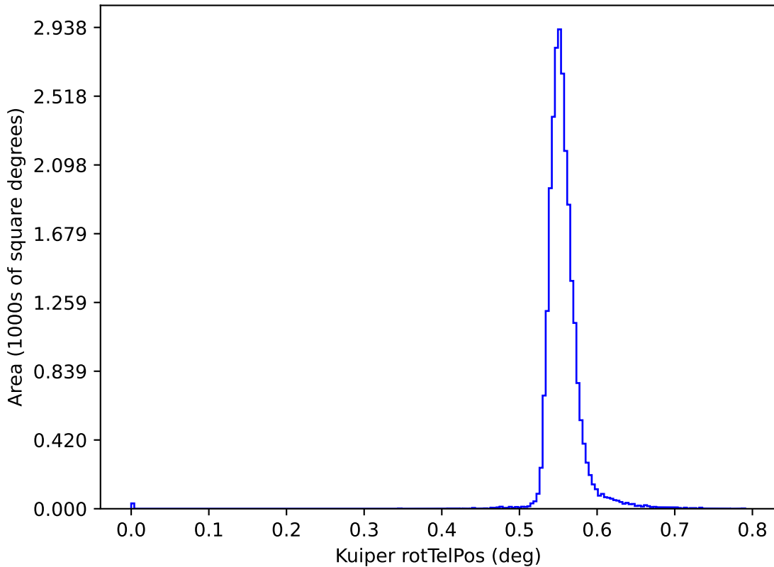
too_elab_r64_d2_griz_v3.4_10yrs y: Kuiper rotTelPos
