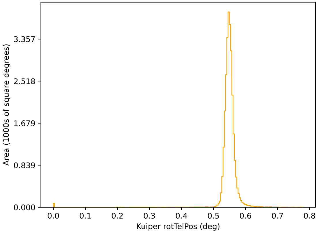
too_elab_r64_d2_griz_v3.4_10yrs r: Kuiper rotTelPos
