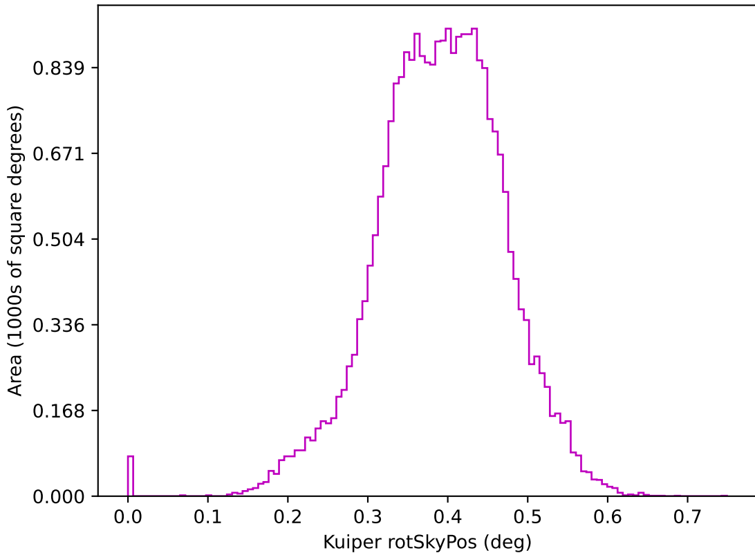
too_elab_r64_d2_griz_v3.4_10yrs z: Kuiper rotSkyPos
