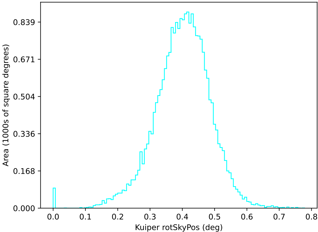
too_elab_r64_d2_griz_v3.4_10yrs u: Kuiper rotSkyPos
