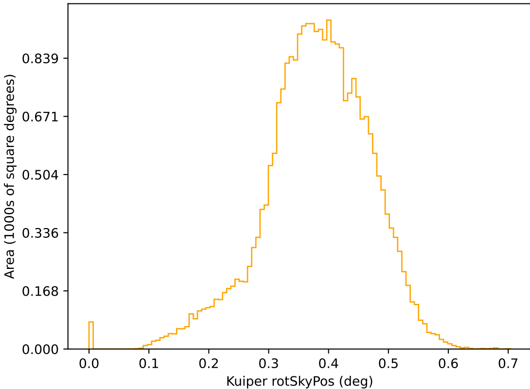
too_elab_r64_d2_griz_v3.4_10yrs r: Kuiper rotSkyPos
