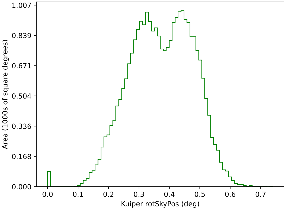
too_elab_r64_d2_griz_v3.4_10yrs g: Kuiper rotSkyPos
