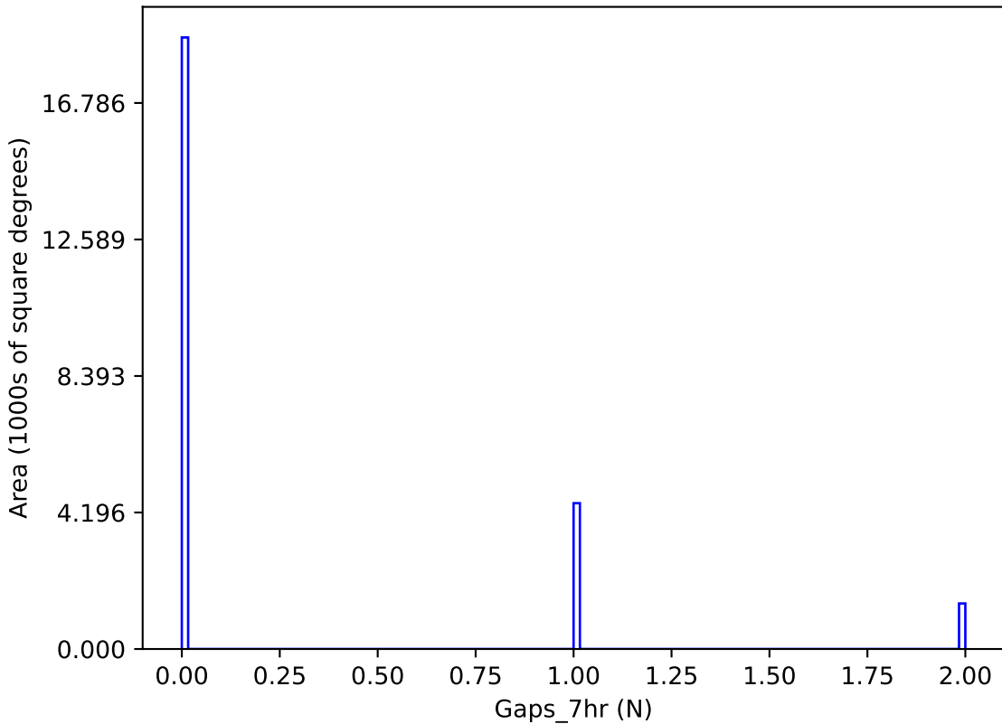
too_elab_r64_d2_griz_v3.4_10yrs y band: Gaps_7hr
