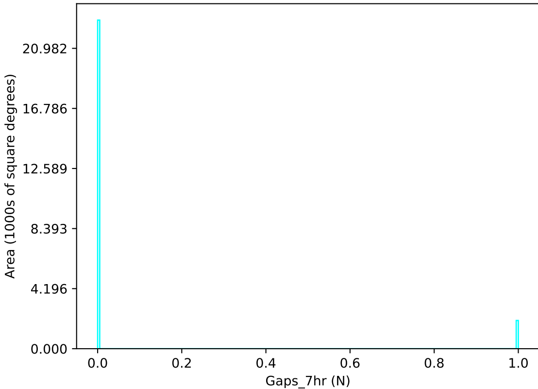
too_elab_r64_d2_griz_v3.4_10yrs u band: Gaps_7hr
