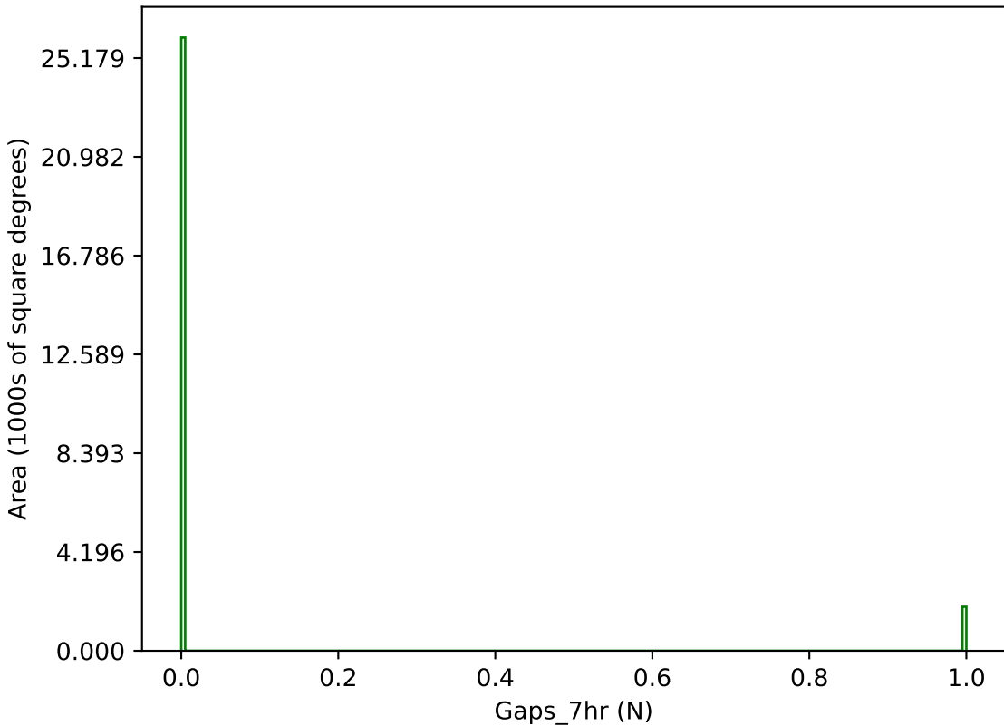
too_elab_r64_d2_griz_v3.4_10yrs g band: Gaps_7hr
