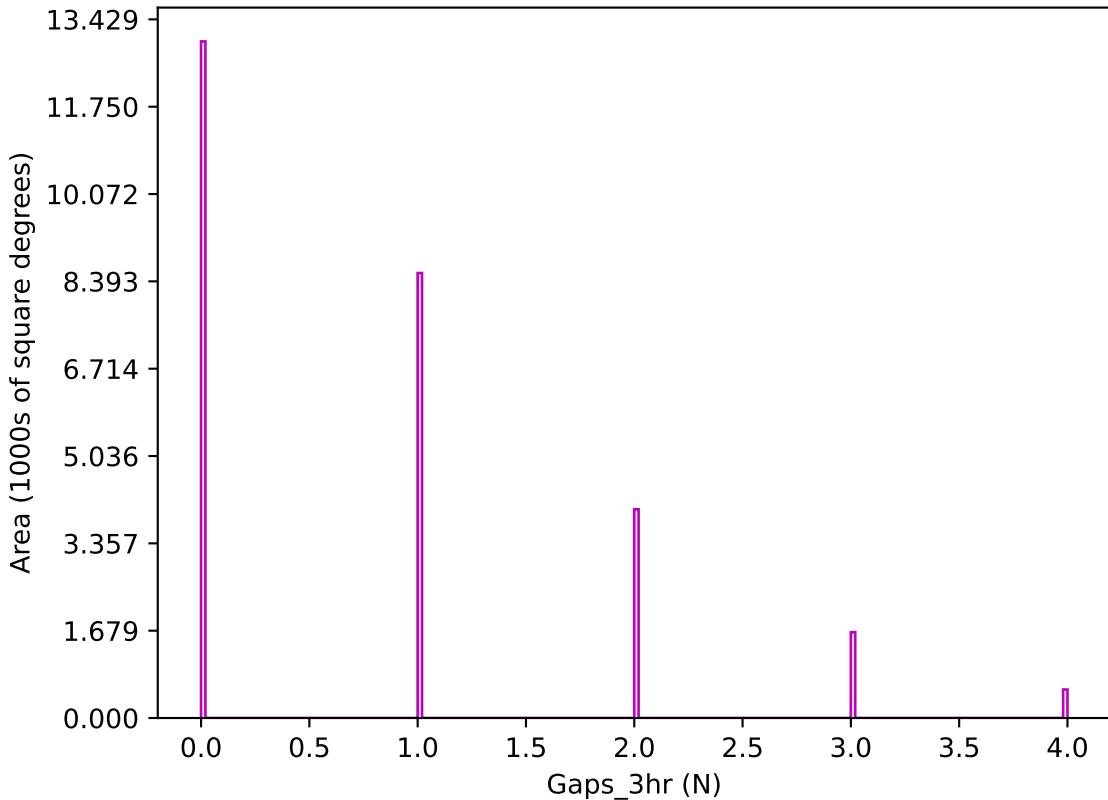
too_elab_r64_d2_griz_v3.4_10yrs z band: Gaps_3hr
