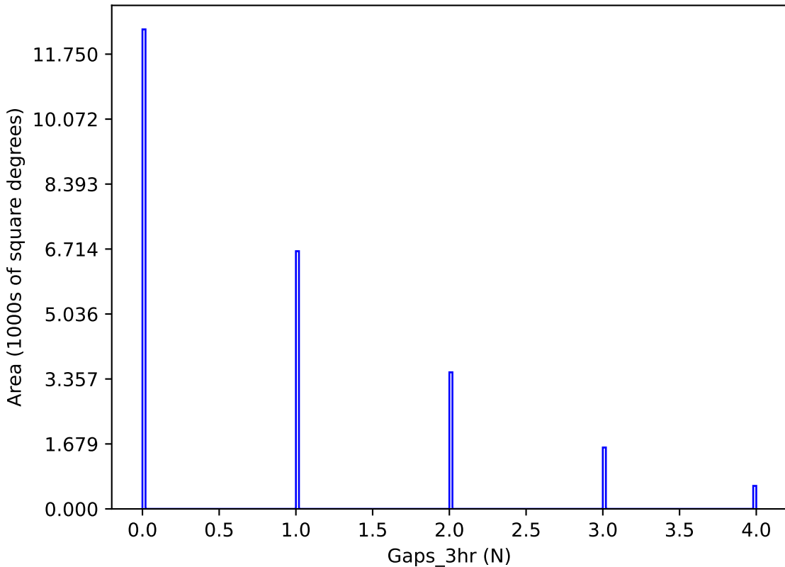
too_elab_r64_d2_griz_v3.4_10yrs y band: Gaps_3hr
