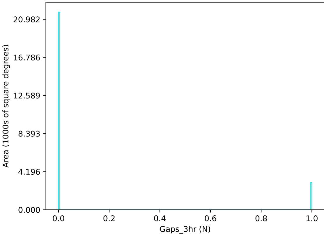
too_elab_r64_d2_griz_v3.4_10yrs u band: Gaps_3hr
