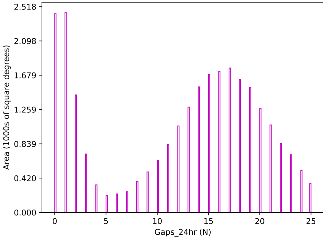
too_elab_r64_d2_griz_v3.4_10yrs z band: Gaps_24hr
