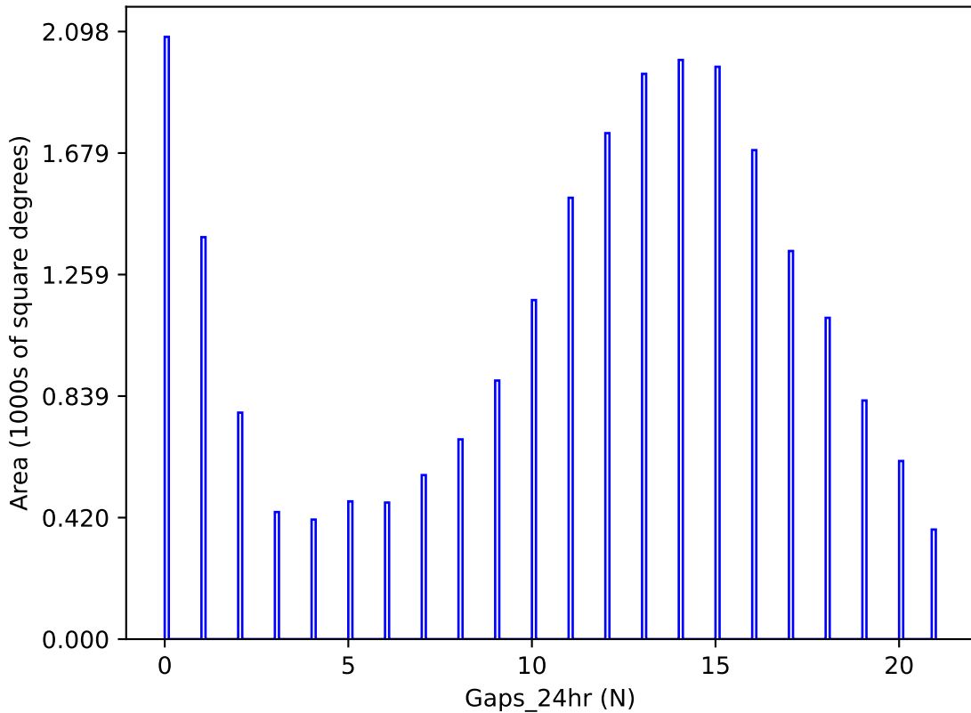
too_elab_r64_d2_griz_v3.4_10yrs y band: Gaps_24hr
