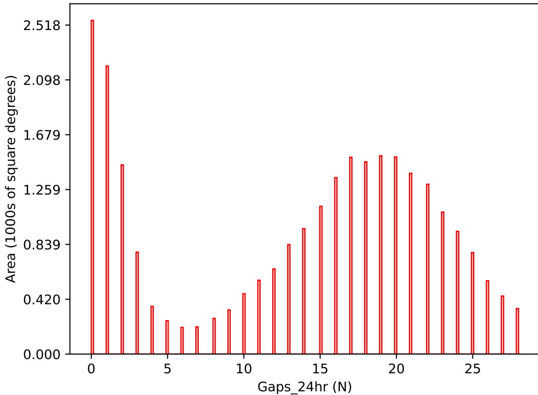
too_elab_r64_d2_griz_v3.4_10yrs i band: Gaps_24hr
