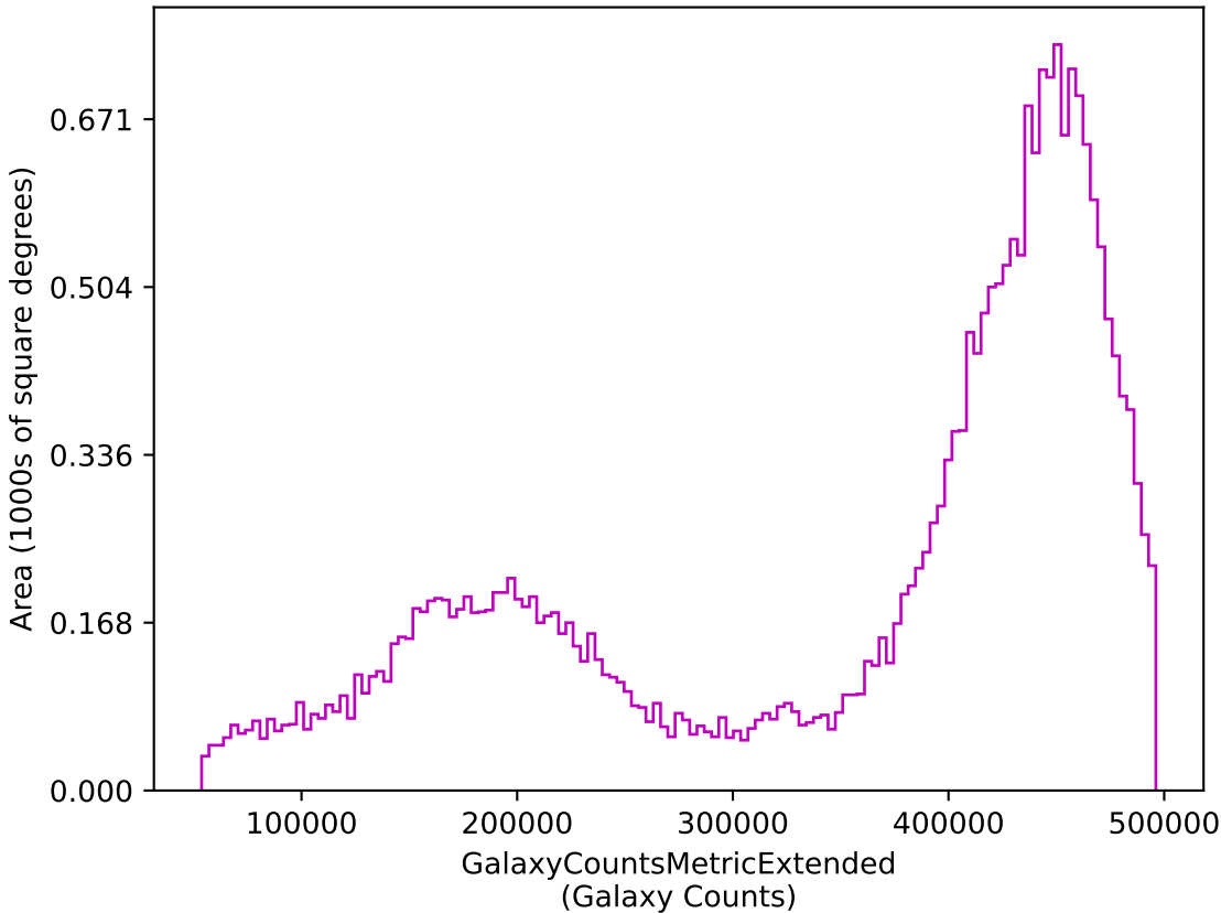
too_elab_r64_d2_griz_v3.4_10yrs z: GalaxyCountsMetricExtended
