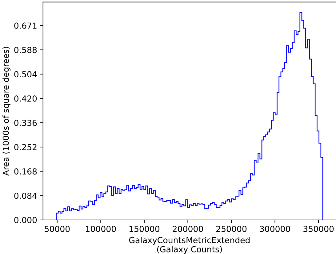
too_elab_r64_d2_griz_v3.4_10yrs y: GalaxyCountsMetricExtended
