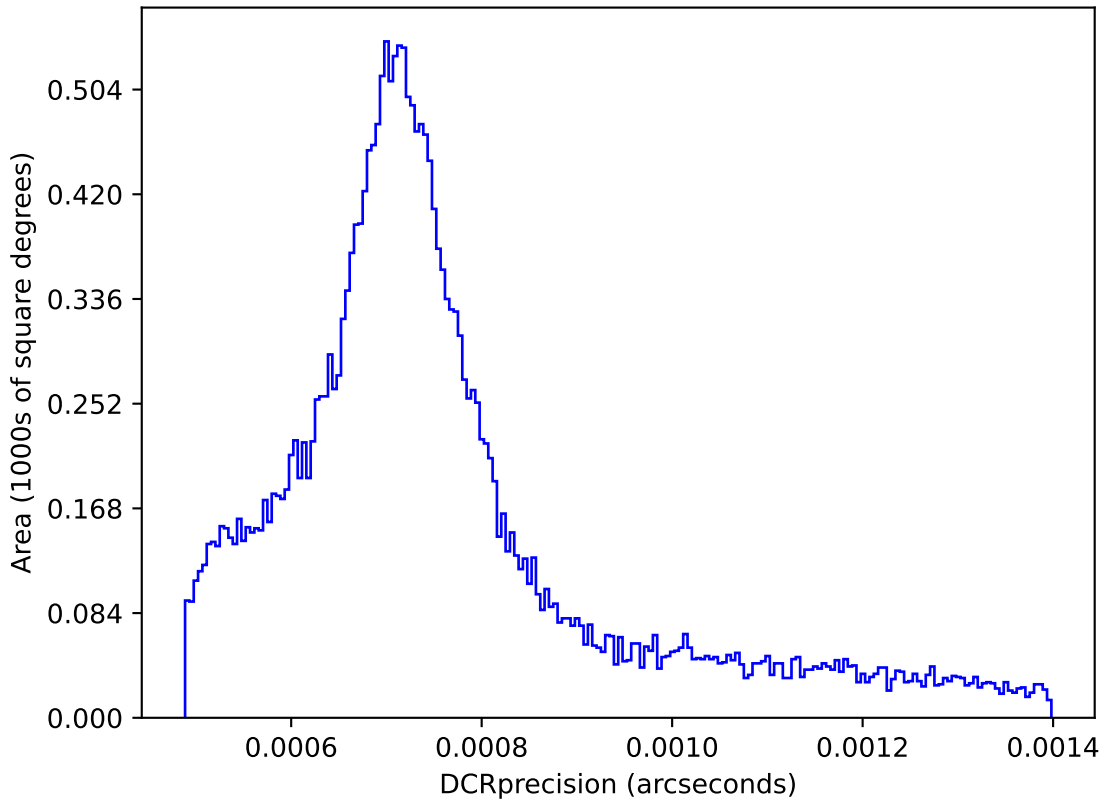
too_elab_r64_d2_griz_v3.4_10yrs : DCRprecision
