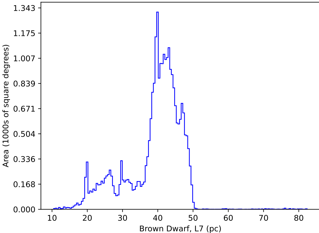
too_elab_r64_d2_griz_v3.4_10yrs : Brown Dwarf, L7
