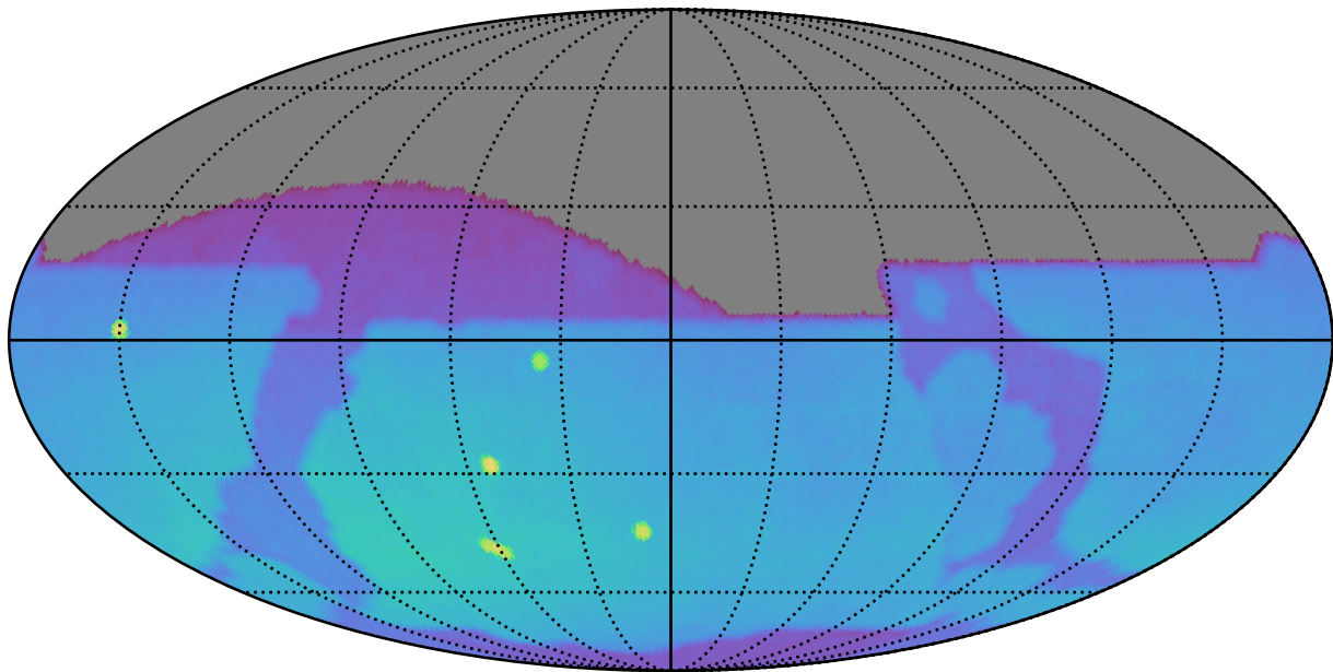
too_elab_r64_d2_griz_v3.4_10yrs : Brown Dwarf, L4
