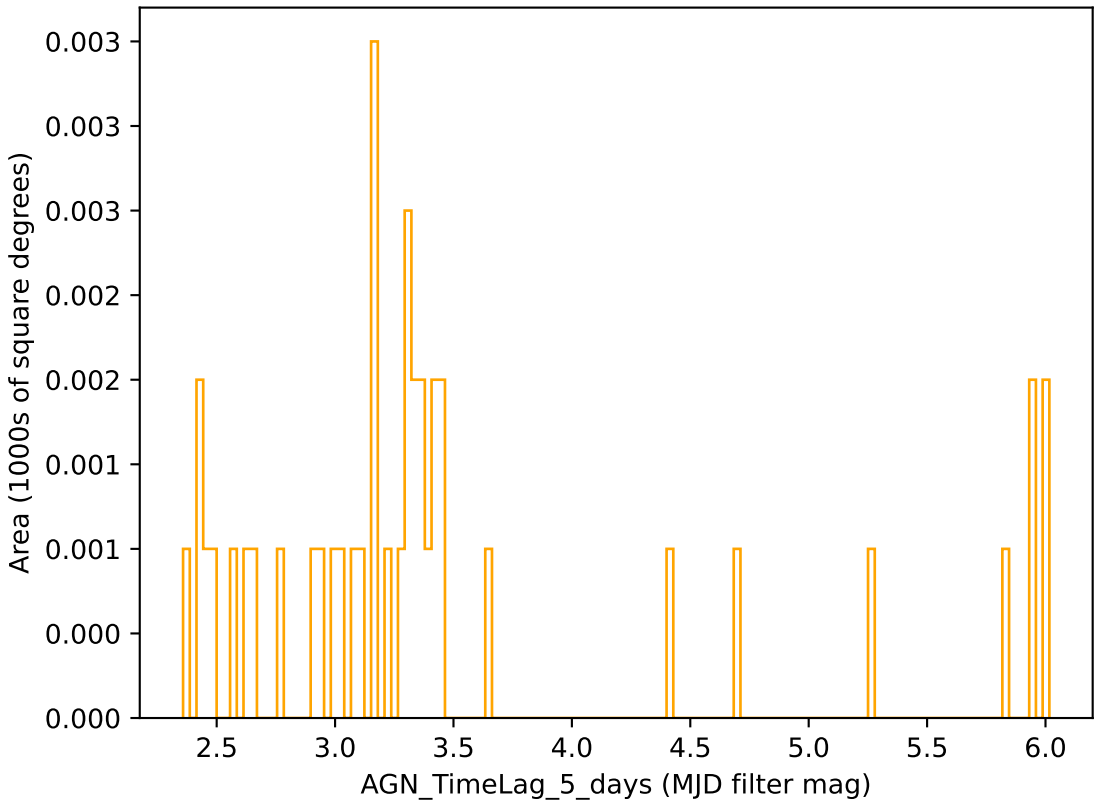
too_elab_r64_d2_griz_v3.4_10yrs r band: AGN_TimeLag_5_days
