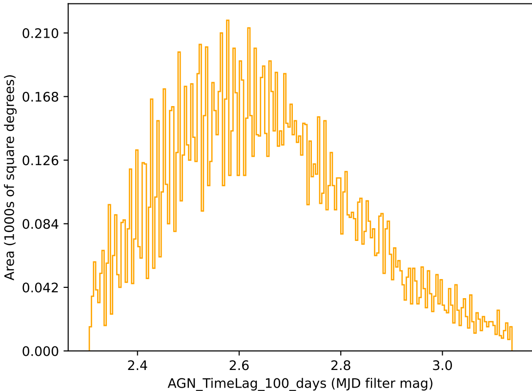
too_elab_r64_d2_griz_v3.4_10yrs r band: AGN_TimeLag_100_days
