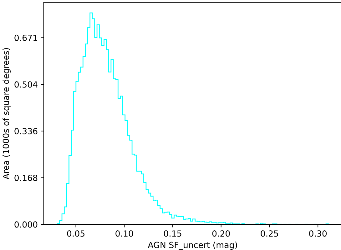
too_elab_r64_d2_griz_v3.4_10yrs u band: AGN SF_uncert
