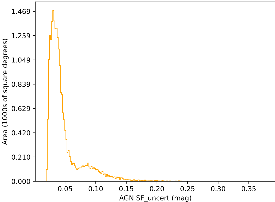
too_elab_r64_d2_griz_v3.4_10yrs r band: AGN SF_uncert
