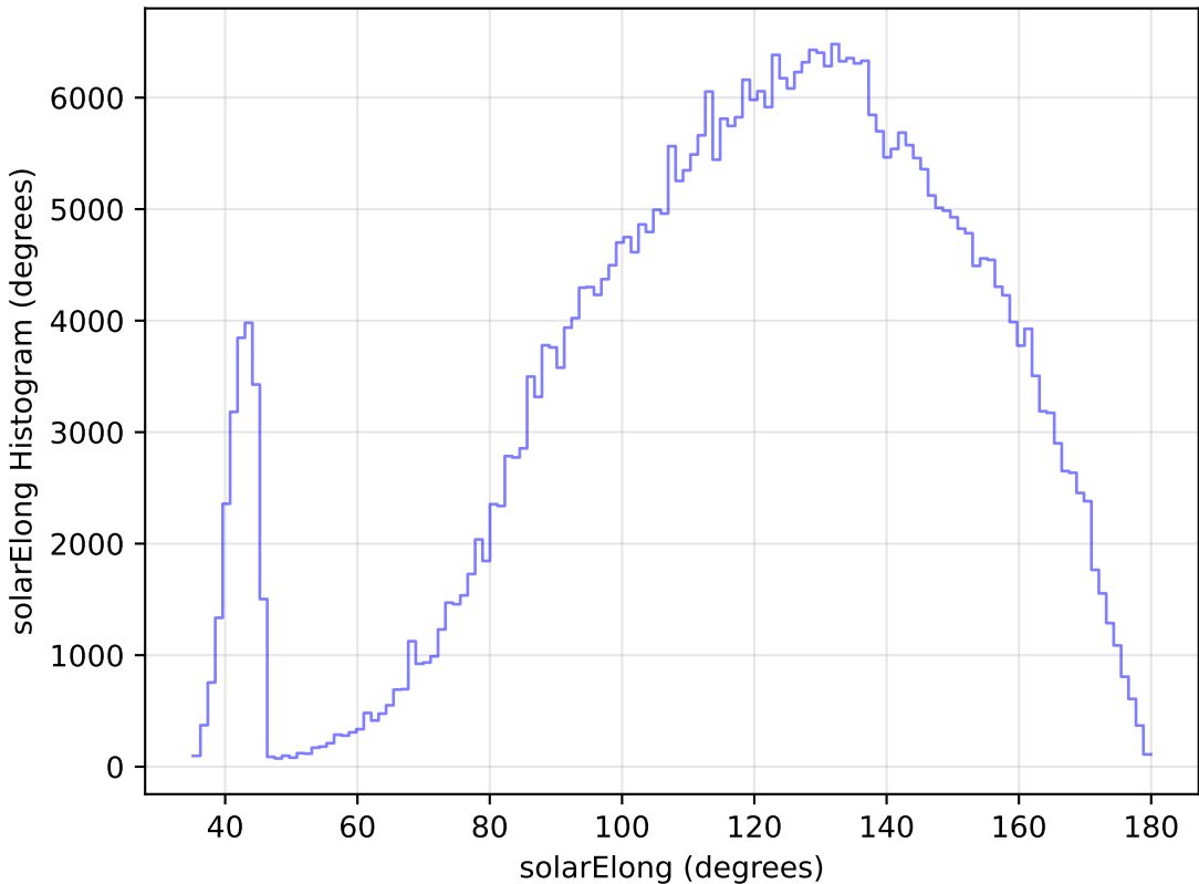
too_elab_r64_d2_griz_v3.4_10yrs WFD z band: solarElong Histogram
