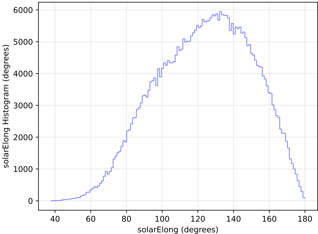
too_elab_r64_d2_griz_v3.4_10yrs WFD y band: solarElong Histogram
