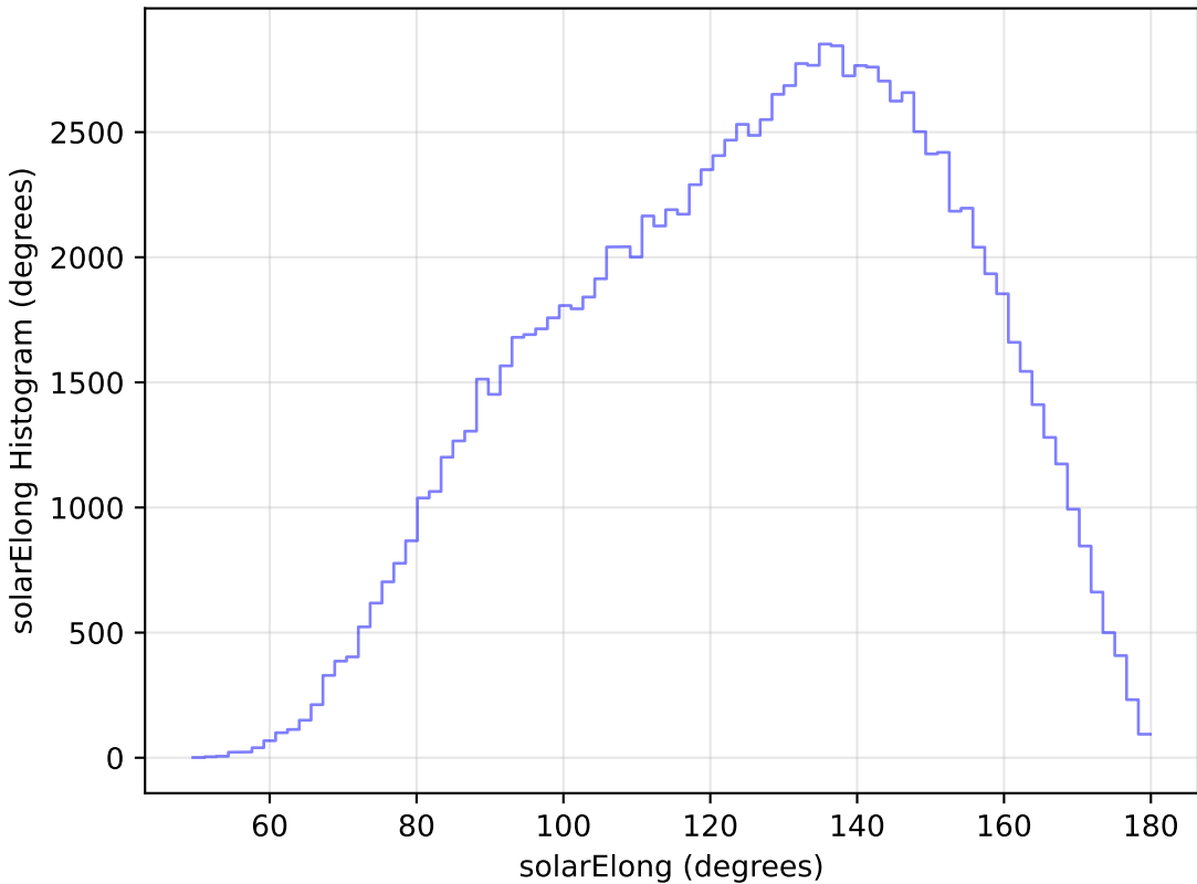
too_elab_r64_d2_griz_v3.4_10yrs WFD u band: solarElong Histogram
