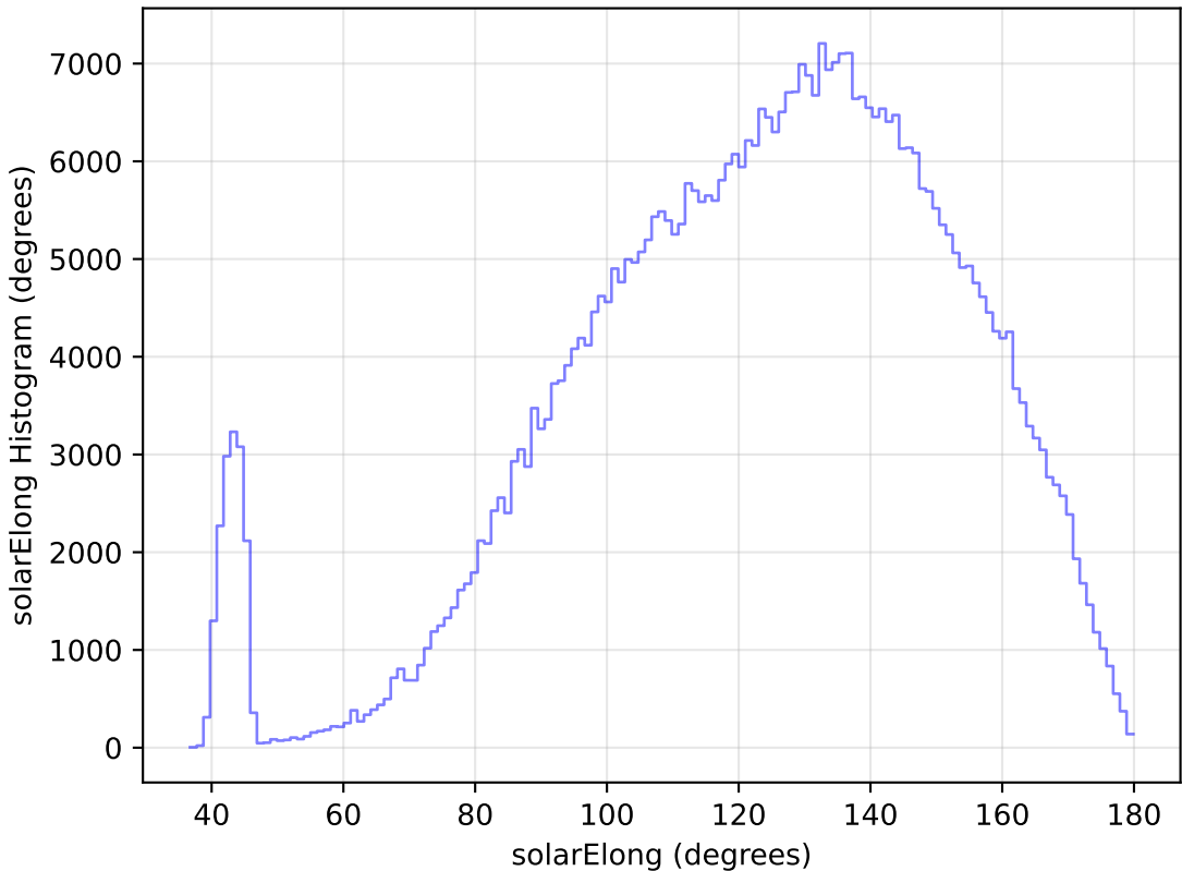
too_elab_r64_d2_griz_v3.4_10yrs WFD r band: solarElong Histogram
