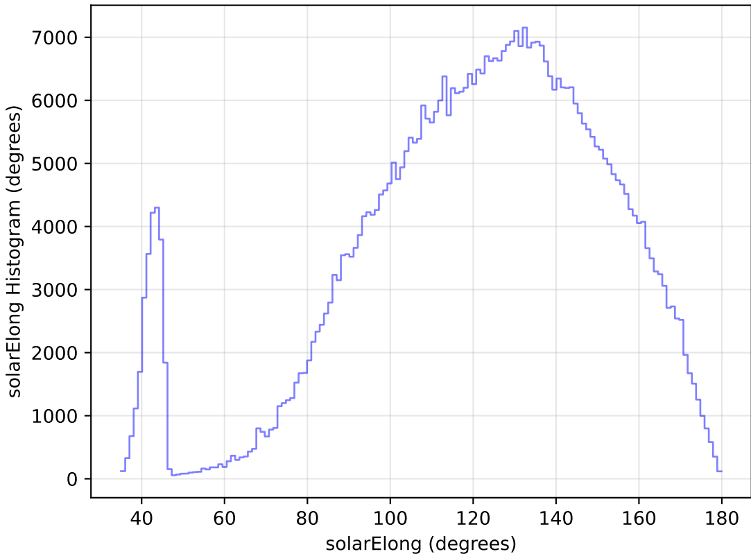
too_elab_r64_d2_griz_v3.4_10yrs WFD i band: solarElong Histogram
