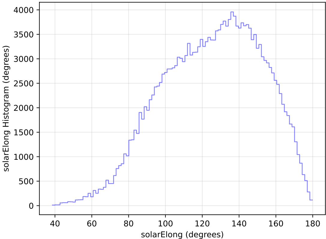
too_elab_r64_d2_griz_v3.4_10yrs WFD g band: solarElong Histogram
