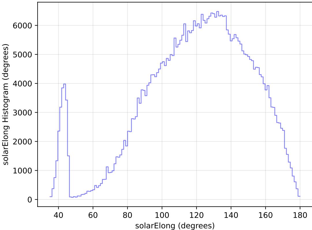
too_elab_r64_d2_griz_v3.4_10yrs All sky z band: solarElong Histogram
