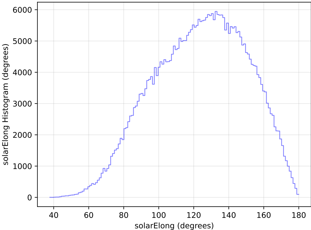
too_elab_r64_d2_griz_v3.4_10yrs All sky y band: solarElong Histogram
