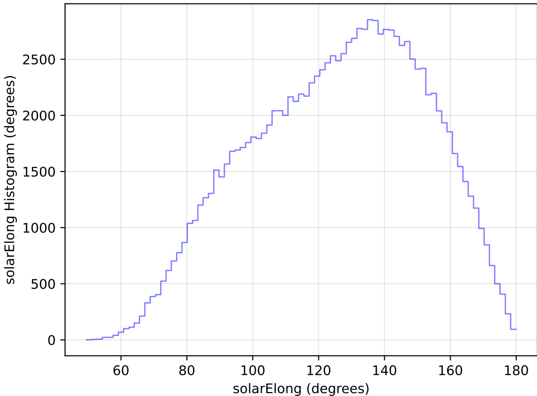
too_elab_r64_d2_griz_v3.4_10yrs All sky u band: solarElong Histogram
