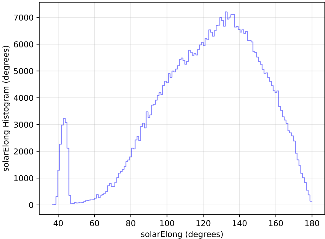
too_elab_r64_d2_griz_v3.4_10yrs All sky r band: solarElong Histogram
