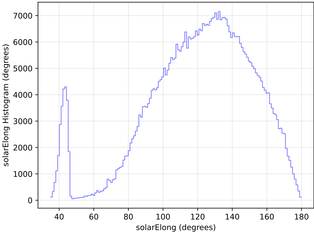
too_elab_r64_d2_griz_v3.4_10yrs All sky i band: solarElong Histogram
