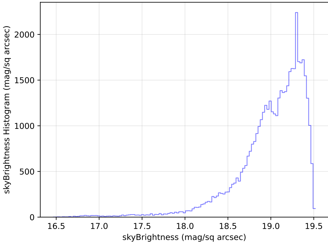
too_elab_r64_d2_griz_v3.4_10yrs Yr 1 z band: skyBrightness Histogram
