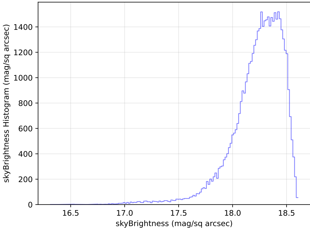
too_elab_r64_d2_griz_v3.4_10yrs Yr 1 y band: skyBrightness Histogram
