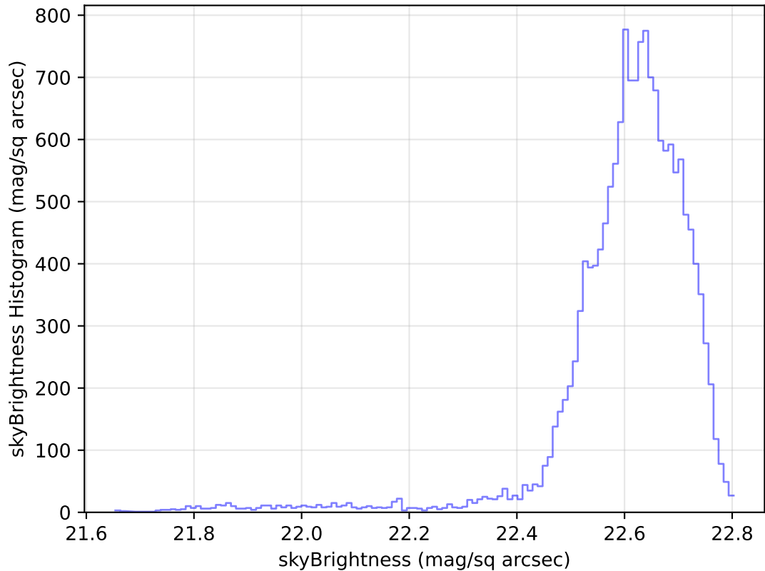
too_elab_r64_d2_griz_v3.4_10yrs Yr 1 u band: skyBrightness Histogram
