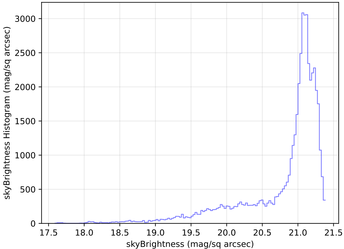
too_elab_r64_d2_griz_v3.4_10yrs Yr 1 r band: skyBrightness Histogram
