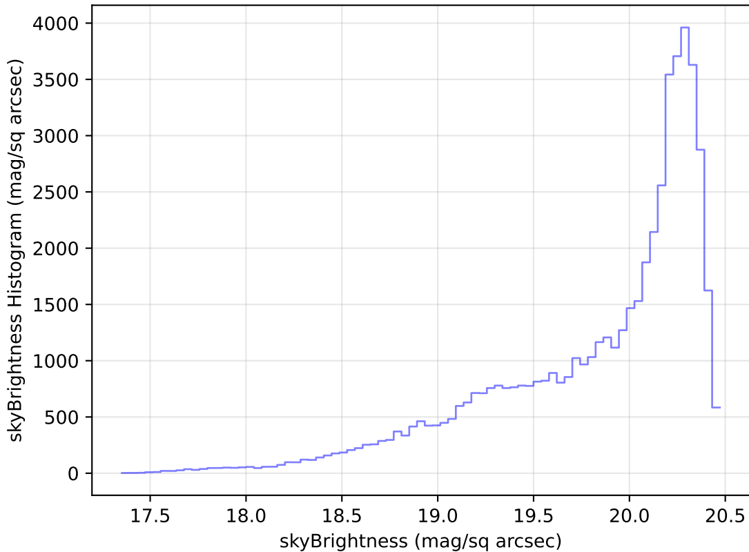
too_elab_r64_d2_griz_v3.4_10yrs Yr 1 i band: skyBrightness Histogram
