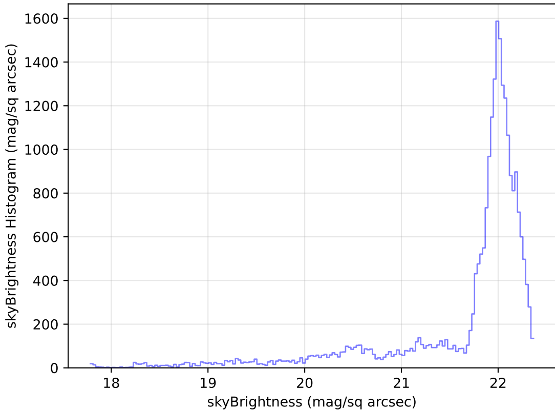
too_elab_r64_d2_griz_v3.4_10yrs Yr 1 g band: skyBrightness Histogram
